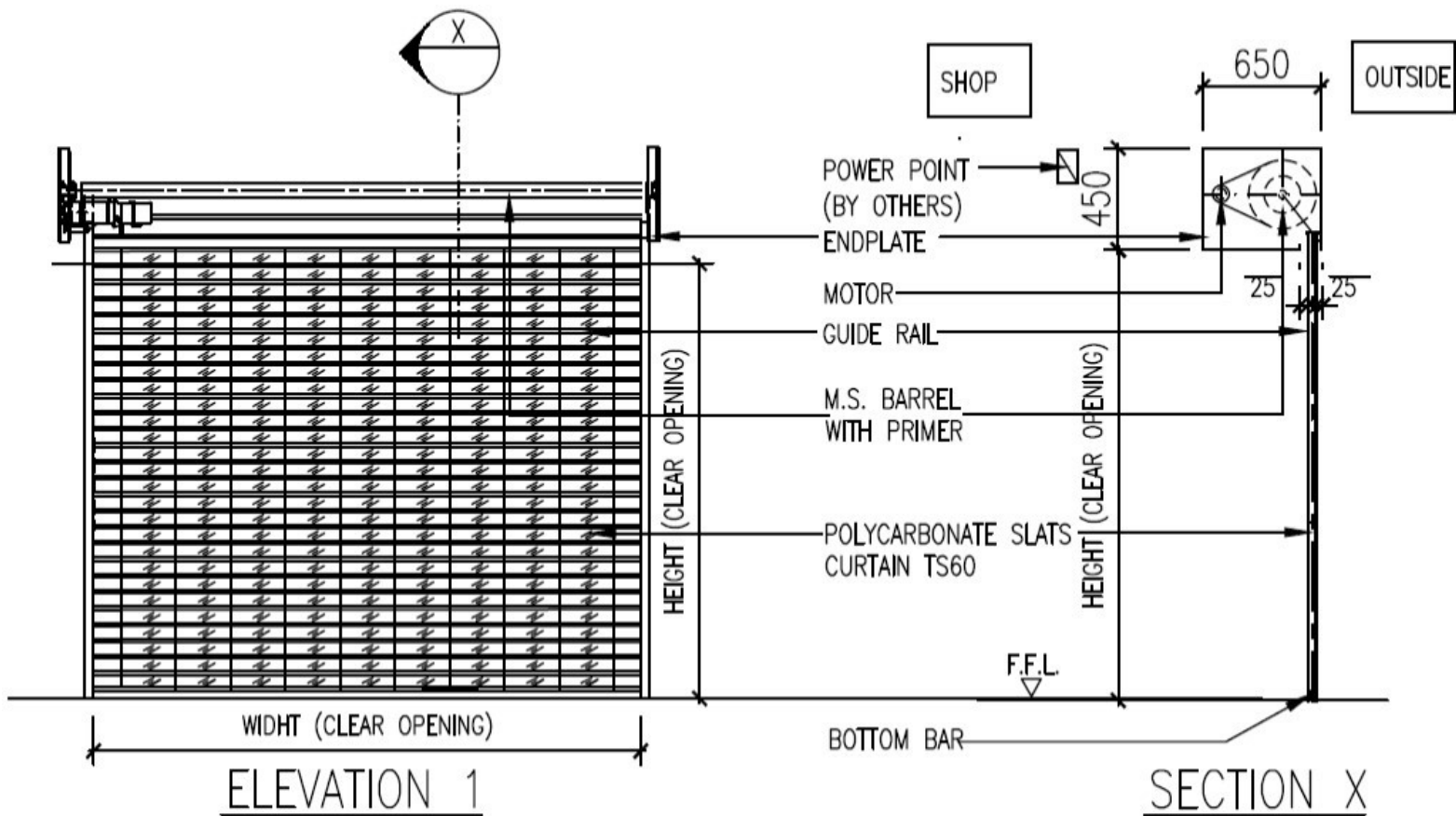
Polycarbonate Panel
